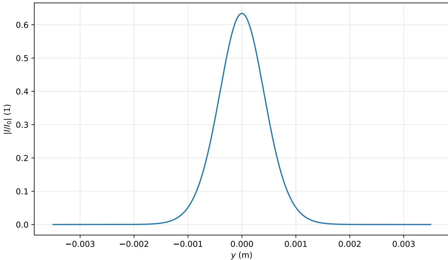
Intensity profile I(x=0, y, z=2.070)/I_0 , \text{Pin}=0.3\text{Pcr} , artificial time
